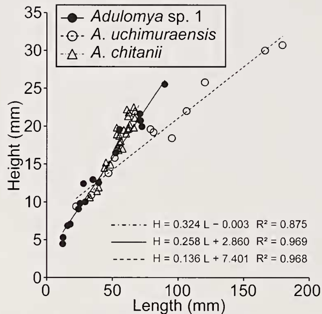
Figure 55. Relationships between shell length and height with growth of Adulomya sp. 1 from Loc. 2, A. uchimuraensis Kuroda, and A. chitani Kanehara. Measurements of A. uchimuraensis and A. chitani are from Kanno et al. (1998) and Amano and Kiel (2011), respectively.
